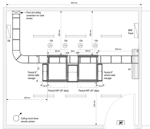
(Diagram 5.3b Drawing MER typical layout arrangement)
