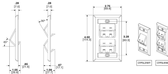
(Diagram 6.4.4a Image approved PANDUIT face plates)
