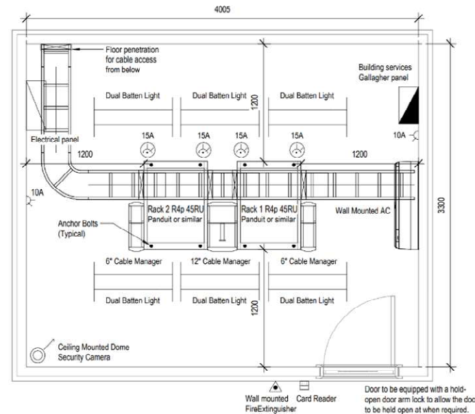
2 ICT Standard Comms Room Type 2
