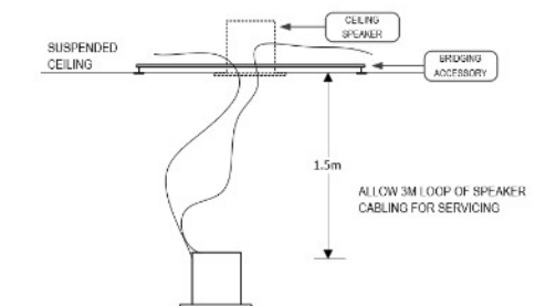
6 CEILING SPEAKER DETAIL
