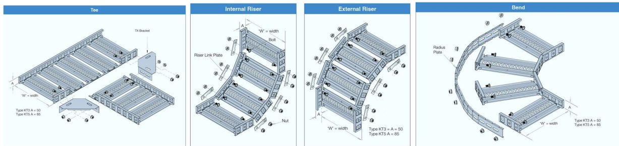
(Diagram 6.2.3.1a Illustration cable trays)
