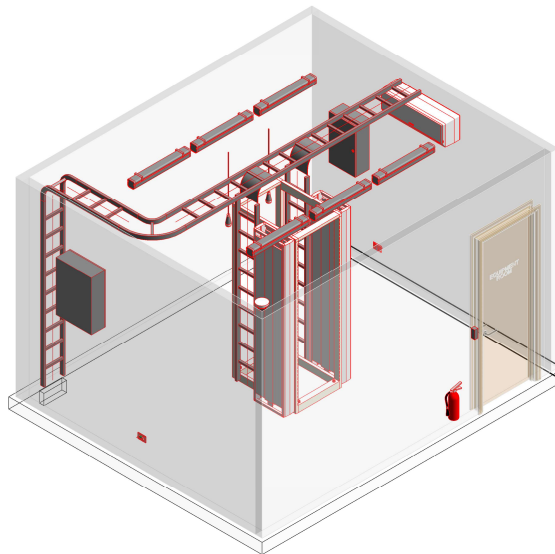
(Diagram 5.1.3a SER Drawing typical arrangement See: Appendices)
