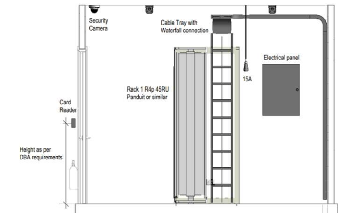
6 West Elevation Type 1
