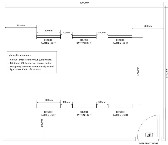
(Diagram 5.2.7a Drawing typical lighting arrangement)
