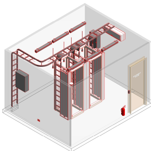
(Diagram 5.1.2a MER Drawing typical arrangement See: Appendices)
