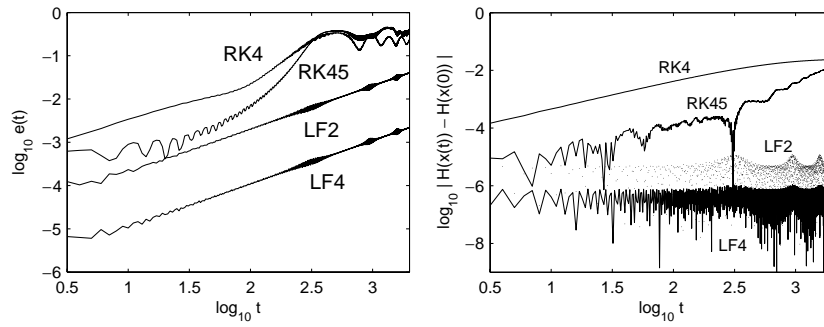
Figure 2. Advantage on quasiperiodic orbits. Global error (left) and energy error (right) for the Hénon–Heiles system with initial condition (q_1, q_2, p_1, p_2) = (0.1, 0.2, 0, 0) , which leads to a quasiperiodic orbit.
