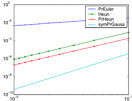
Figure 4.4: Order plot of the projected Euler, Heun, projected Heun and symmetric projected 2-stage Gauss method for the Duffing equation.
