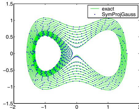
Figure 4.3: Symmetric projected 2-stage Gauss method ( h = 0.25 ).
