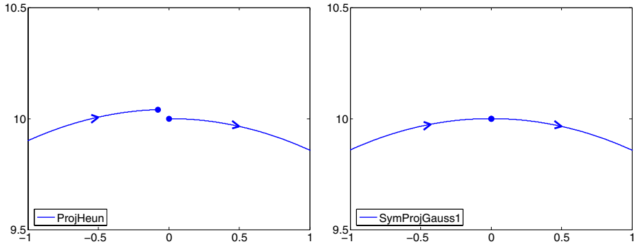
Figure 4.7: Projected Heun method ( h = 0.5 ), symmetric projected one-stage Gauss method ( h = 0.5 ).
