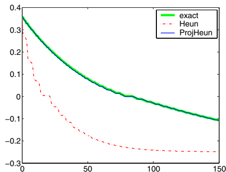
Figure 4.5: Rate of dissipation of the Heun and projected Heun method for the Duffing equation. Step size h = 0.5 , starting value (1.6, 0) and time = [0, 150] .
