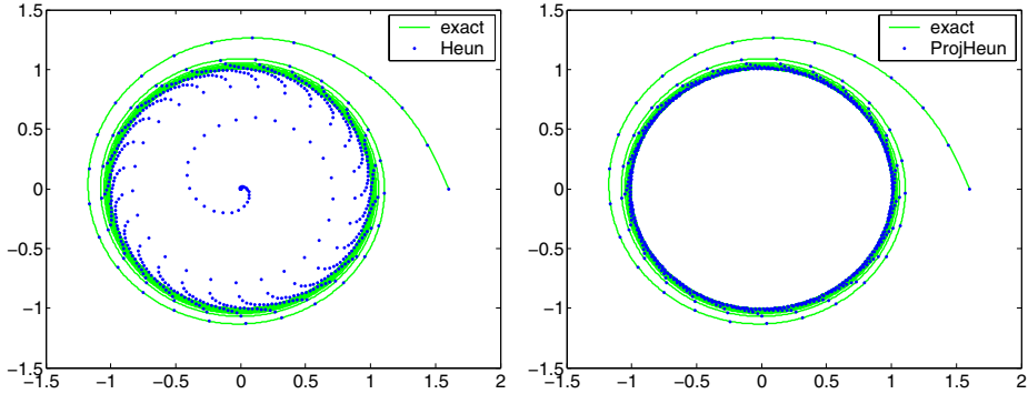
Figure 4.6: Heun method ( h = 0.25 ), projected Heun method ( h = 0.25 ).
