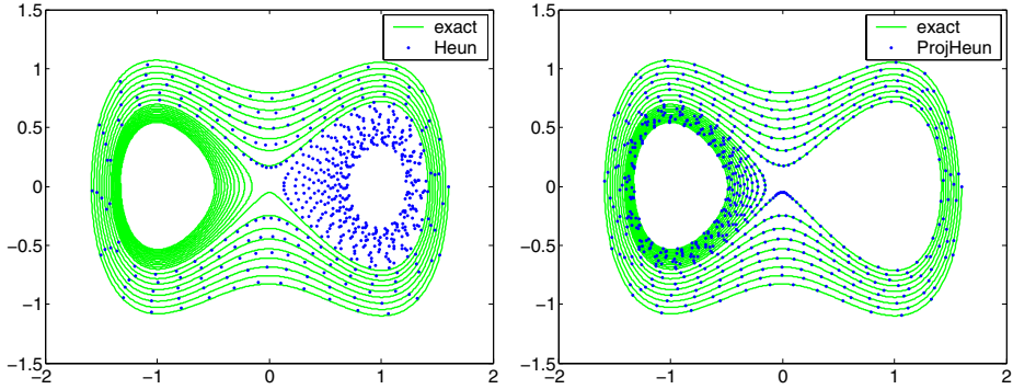
Figure 4.2: Heun method ( h = 0.25 ), projected Heun method ( h = 0.25 ).
