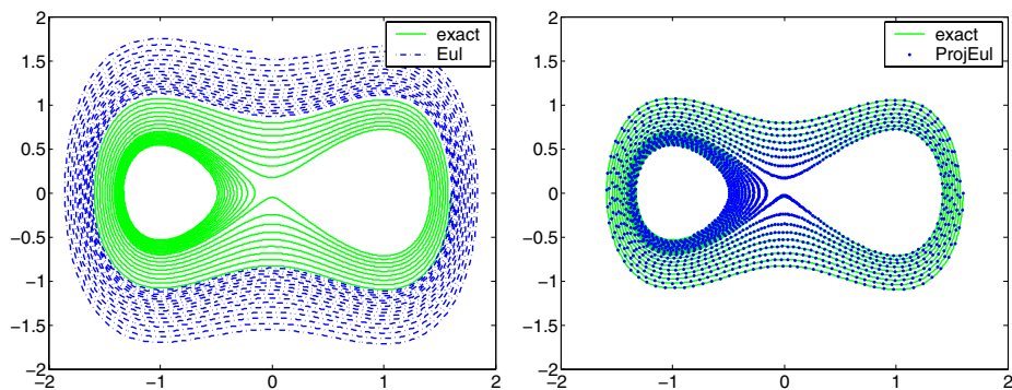
Figure 4.1: Euler method ( h = 0.01 ) and projected Euler method ( h = 0.08 ).
