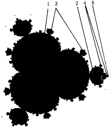
Figure 1. The Mandelset M(\lambda - z^4, 0) of the elementary quartic polynomial. The integer label gives the period of some of the hyperbolic components.
