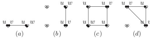
Figure 15. The stencil of the Boussinesq system (32).
