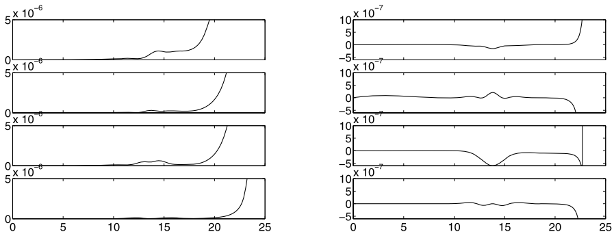
Fig. 5 The global truncation error in y (left), and the error in the Hamiltonian (right) against time t after the Hamiltonian Hopf bifurcation at \lambda = 0.5 . The integrators included are gauss4 (top), hochost4 (second), exprk4 (third) and method (bottom)
