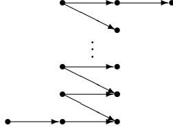
FIGURE 2. The directed graph \mathbf{Z}_n .
