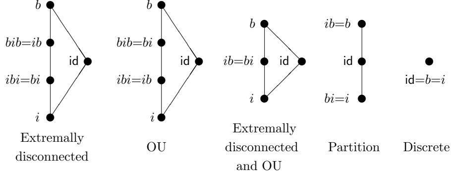
FIGURE 2.1. Orderings on 5 possible Kuratowski monoids.
