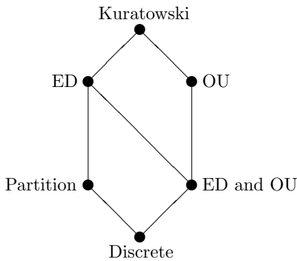
FIGURE 2.3. The six different Kuratowski monoids for topological spaces.
