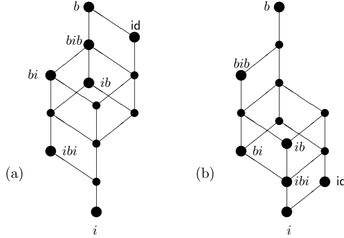
FIGURE 4.1. The 13 different operators produced by b , i and \wedge and by b , i and \vee .
