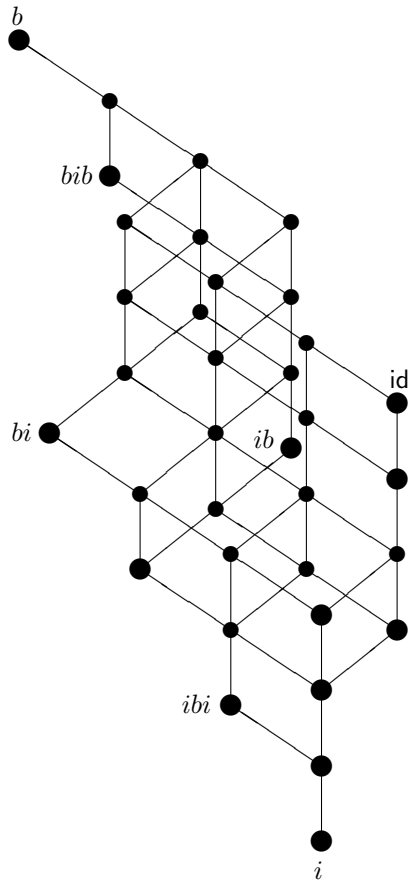
FIGURE 4.2. The 35 different operators produced from b, i, \wedge and \vee .
