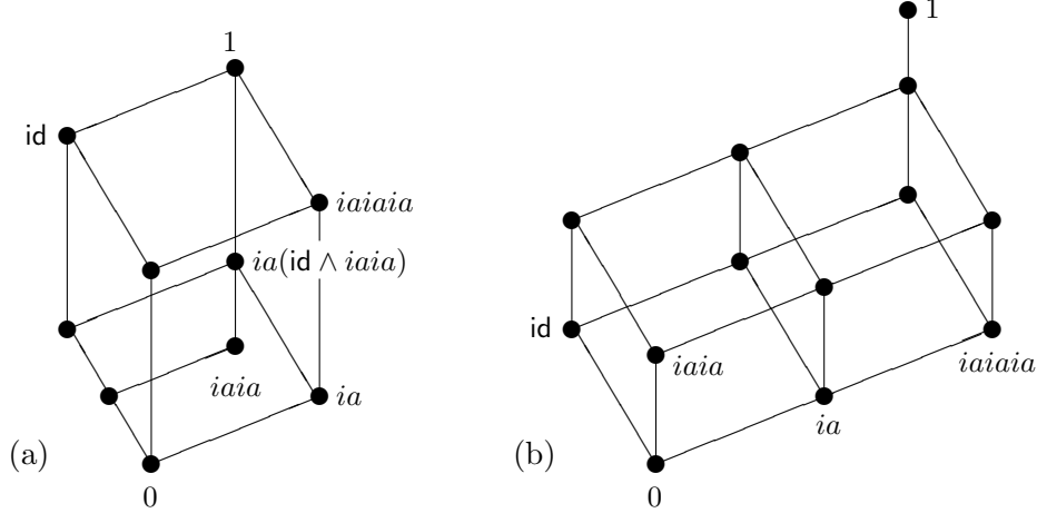
FIGURE 4.3. The 10 operators produced from ia and \wedge and the 13 produced from ia and \vee .
