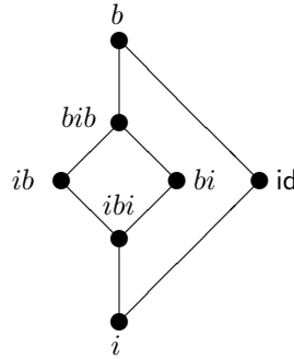
FIGURE 1.1. The seven different operators using b and i .
