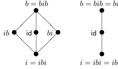
FIGURE 2.2. Two nearly possible Kuratowski monoids.
