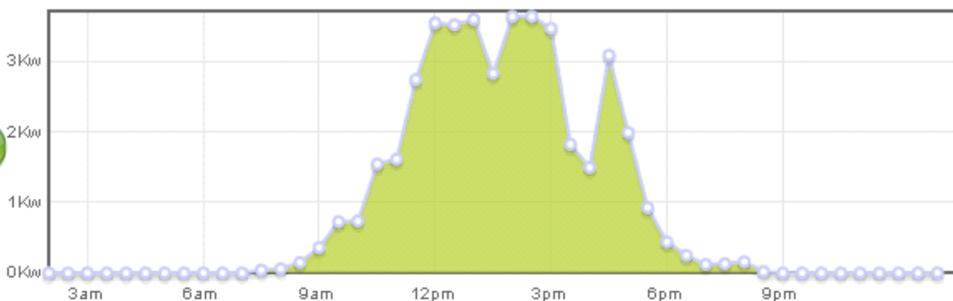
Exported Energy on 2008-12-01
